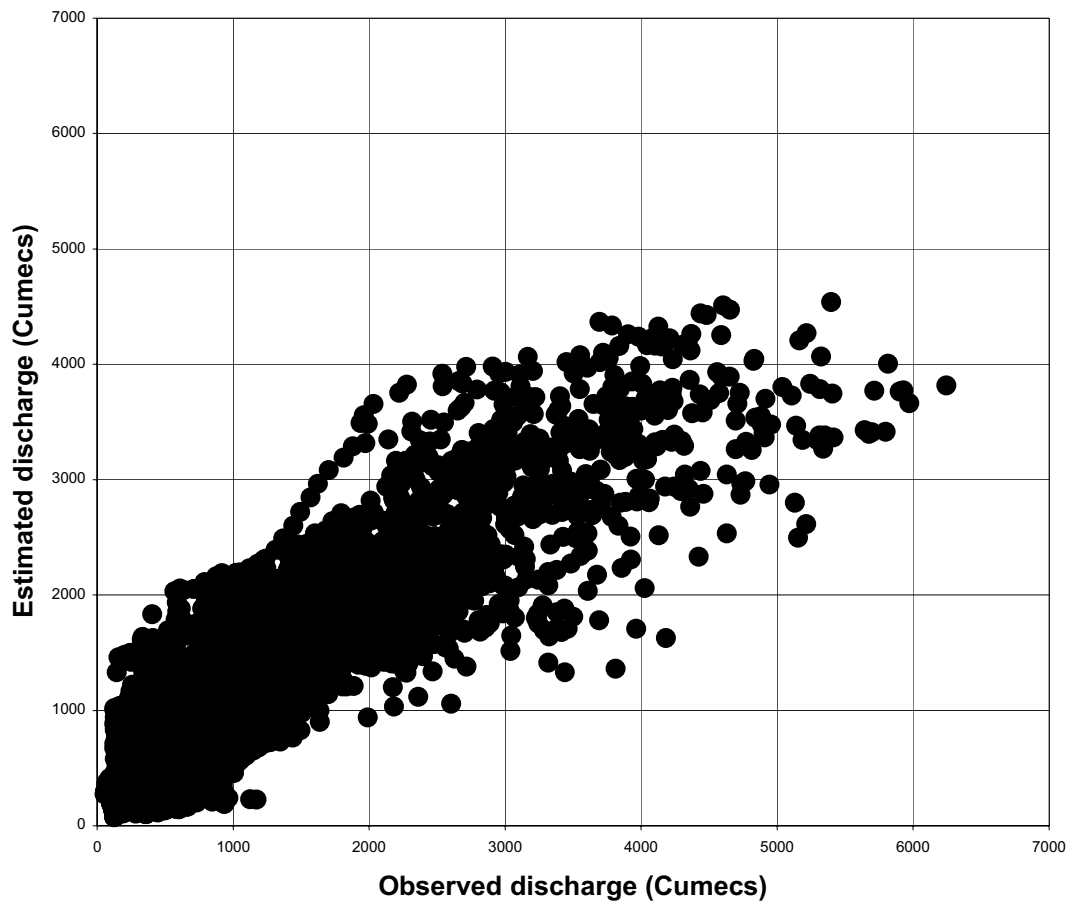
A scatter diagram for observed and estimated flows using Simple Linear Model (SLM) at Stiegler's Gorge (1k3). Inputs: 1ka3, 1kb17 and Average rainfall over intervening catchment
