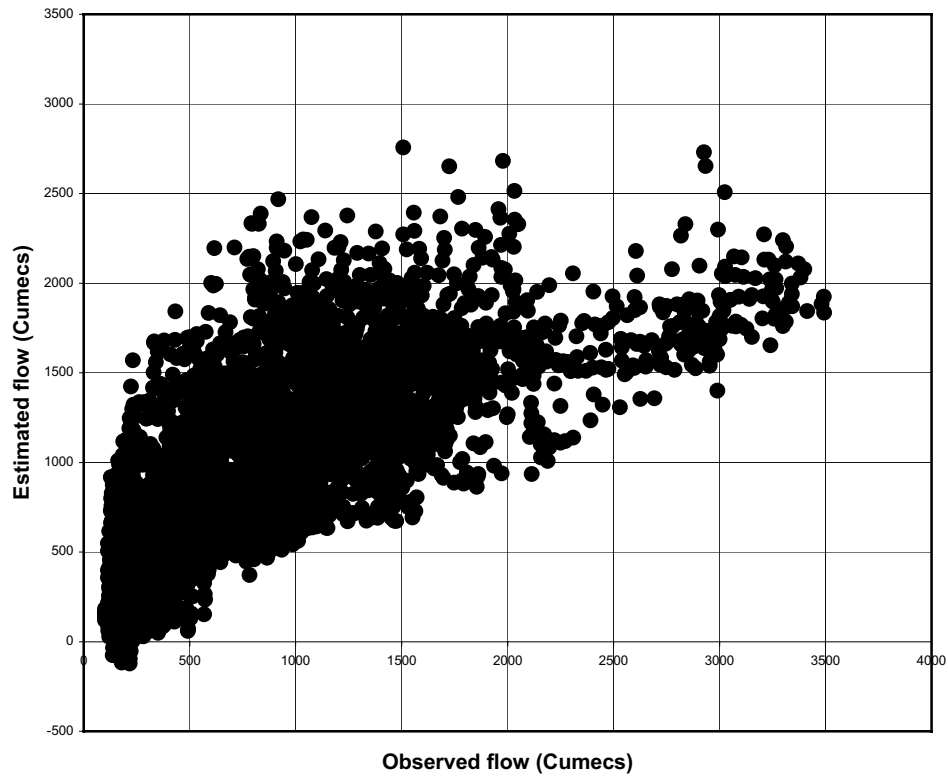
A scatter plot for observed and estimated flows using Linear Varying Gain Factor Model (LVGFM) at Kilombero (1kb17). Inputs: 1kb14, 1kb4, 1kb15a and Intervening catchment average rainfall
