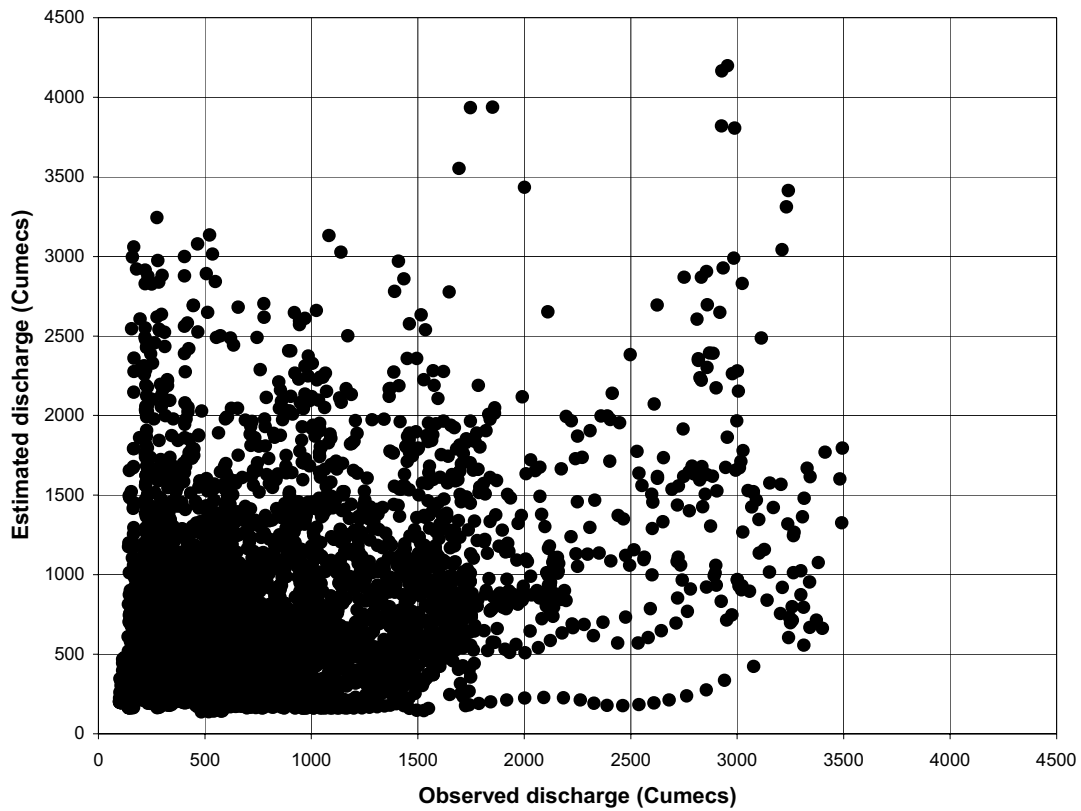
A scatter diagram of observed and estimated flows using HEC-HMS at Kilombero (1kb17). Inputs: 1kb4, 1kb14, 1kb15a and Intervening catchment average rainfall
