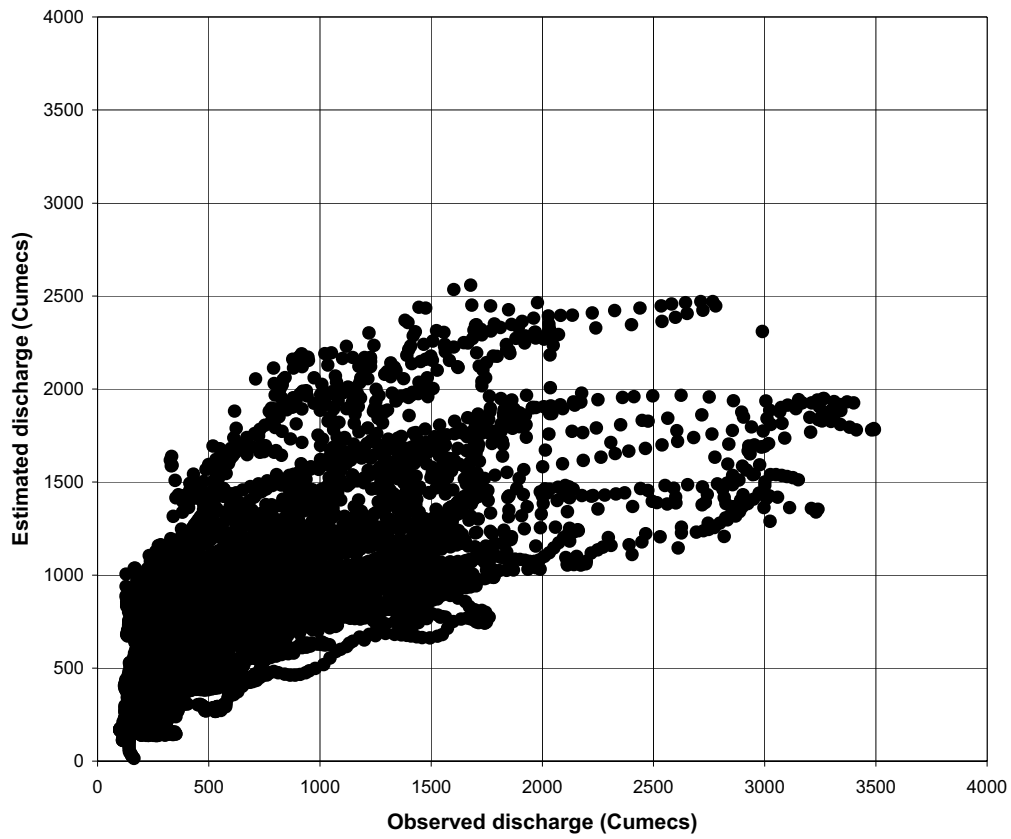
A scatter diagram for observed and estimated flows using Simple Linear Model (SLM) at Kilombero (1kb17). Inputs: 1kb4, 1kb14, 1kb15a and Intervening catchment average rainfall
