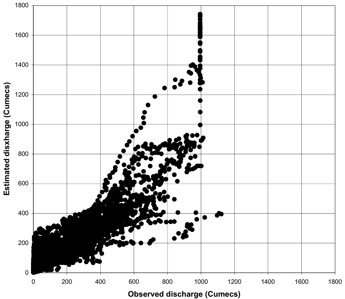
A scatter plot for observed and estimated flows using Simple Linear Model (SLM) at Mtera (1ka5). Inputs: 1ka31, 1ka59 and 1ka42
