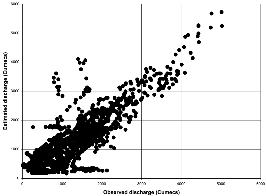
A scatter diagram for observed and estimated flows using Simple Linear Model (SLM) at Mloka (1k4). Input: Observed flows at Stiegler's Gorge (1k3)
