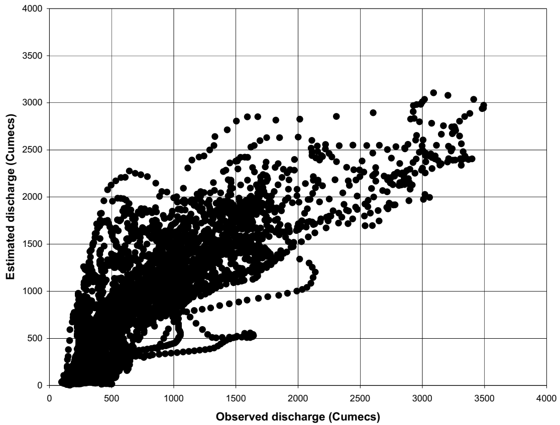
A scatter diagram of observed and estimated flows using Soil Moisture Accounting and Routing model (SMAR) at Kilombero (1kb17). Inputs: Average catchment rainfall and potential evaporation
