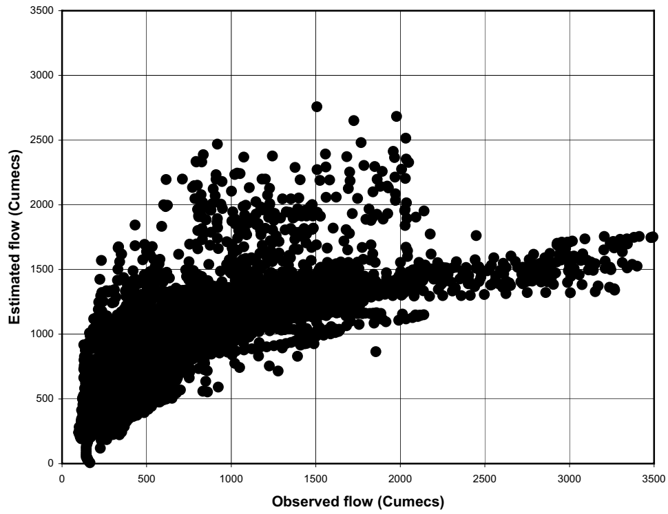
A scatter diagram of observed and estimated flow using Simple Linear Model (SLM) at Kilombero (1kb17). Input: Catchment average rainfall
