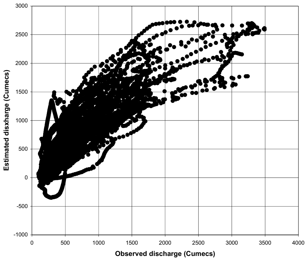
A scatter diagram for observed and estimated flows using Linear Perturbation Model at Kilombero (1kb17). Inputs: 1kb4, 1kb14, 1kb15a and Intervening catchment average rainfall
