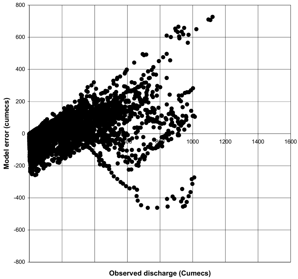
An error diagram for Simple Linear Model (SLM) in estimating flows at Mtera (1ka5). Inputs: 1ka31, 1ka59 and 1ka42
