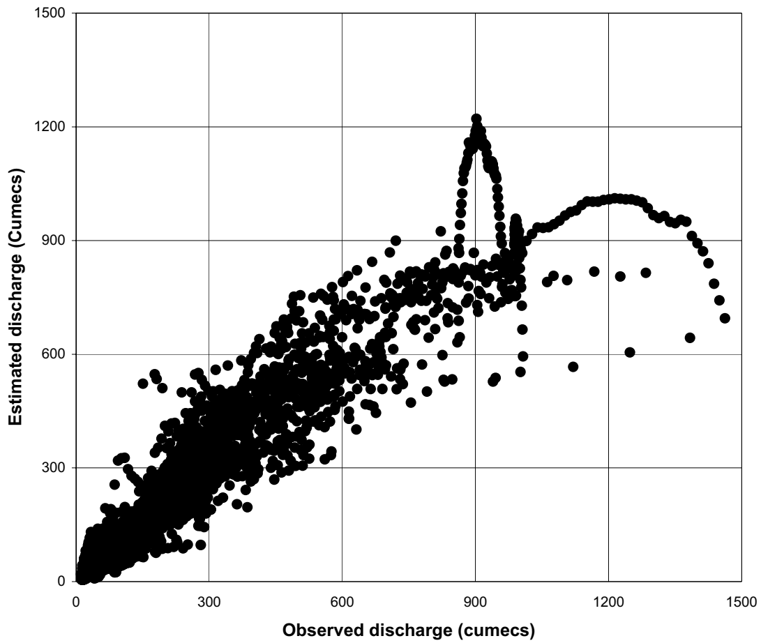
A scatter diagram for observed and estimated flows using Simple Linear Model (SLM) at Kidatu (1ka3). Inputs: 1ka37a, 1ka38, 1ka5 (Mtera) and Intervening catchment average rainfall
