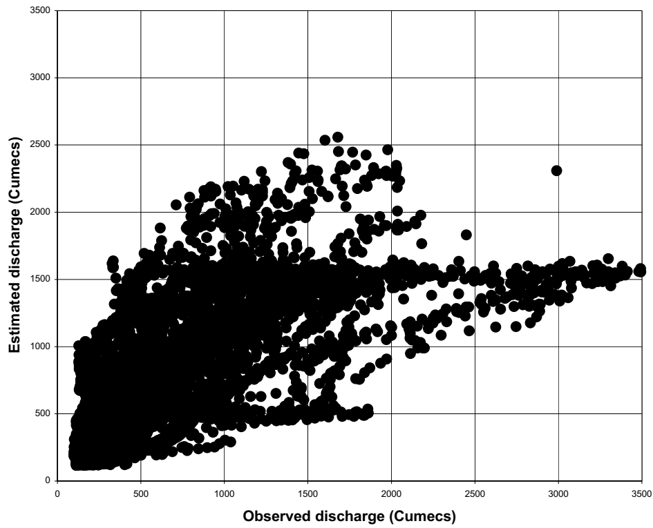
A scatter diagram of observed and estimated flows using Linear Varying Gain Factor Model (LVGFM) at Kilombero (1kb17). Input: Catchment average rainfall
